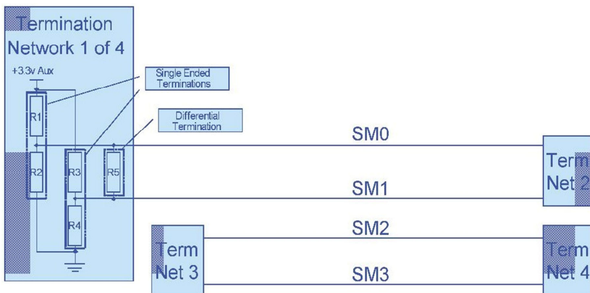
Figure 4-2 SM Bus Terminations
