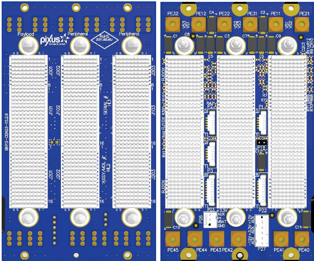
Figure 2-1: Connector Locations
