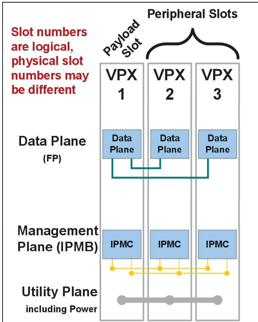
Figure 4-1 Backplane Topology
