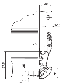
Detail X
