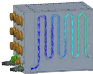
VITA 48.4 and Liquid Through Sidewalls Solutions
