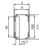
Section B – B Type I, 6U
