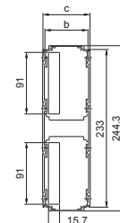
Section B – B Type I, 6U
