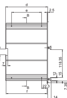
Section A – A Board depth 160 mm
