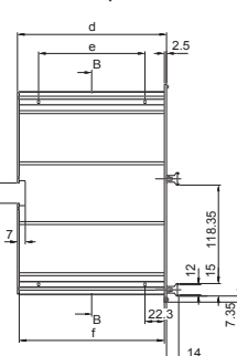
Section A – A Board depth 160 mm
