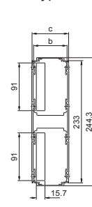
Section B – B Type I, 6U
