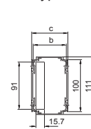
Section B – B Type I, 3U
