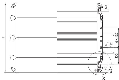
RiCase 269.2 mm (1/2 19")
