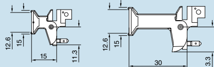
Type I extractor handle Type II extractor handle
