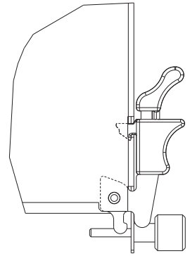
Handle/microswitch
